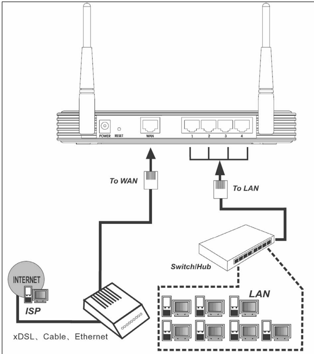
Figure 2-1 Hardware Installation of the TL-WR841ND Wireless N Router
